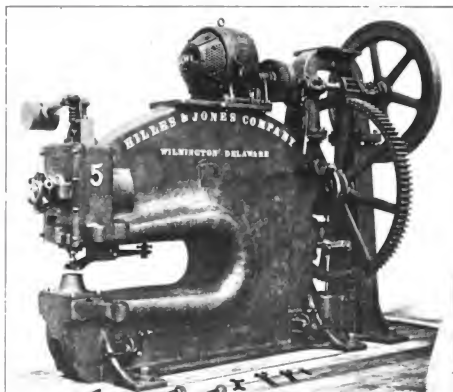
Fig. 4991. Deep Throat Punching Machine. Hilles & Jones Co.
